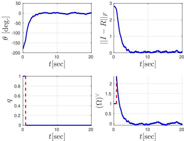
Fig. 3. The top left and top right plots show the errors converging to zero. The bottom left plot shows the logic variable switching from 1 to 0 around t = 1 secs and the bottom right plot shows the control input.
