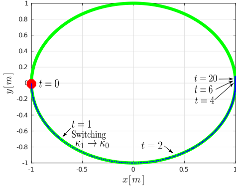
Fig. 2. Hybrid control scheme achieves global asymptotic stability on \mathbb{S}^1 .
