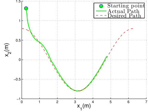
(a) Chameleon R100 following the sinusoidal path.
