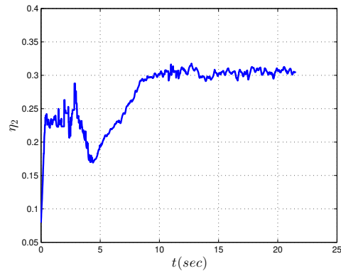
Fig. 5: The Chameleon R100 maintaining a desired speed of 0.3 m/sec along the sinusoidal path.
