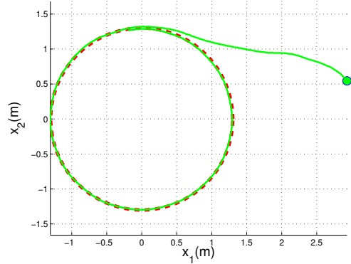
(a) Chameleon R100 following the circular path.
